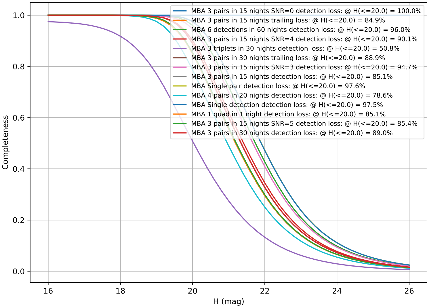
roll_uniform_early_half_mjdp253_v3.4_10yrs: CumulativeCompleteness
