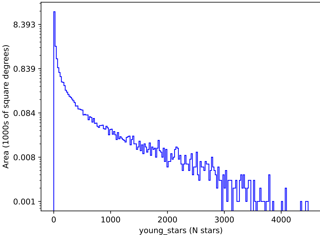
roll_uniform_early_half_mjdp253_v3.4_10yrs : young_stars
