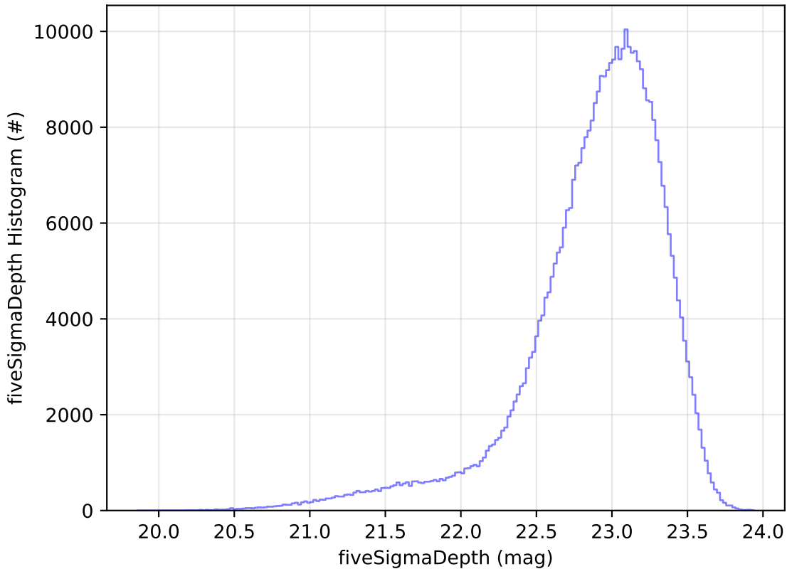
roll_uniform_early_half_mjdp253_v3.4_10yrs z: fiveSigmaDepth Histogram
