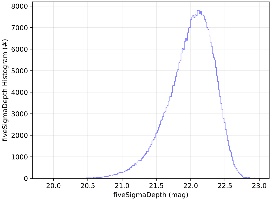
roll_uniform_early_half_mjdp253_v3.4_10yrs y: fiveSigmaDepth Histogram
