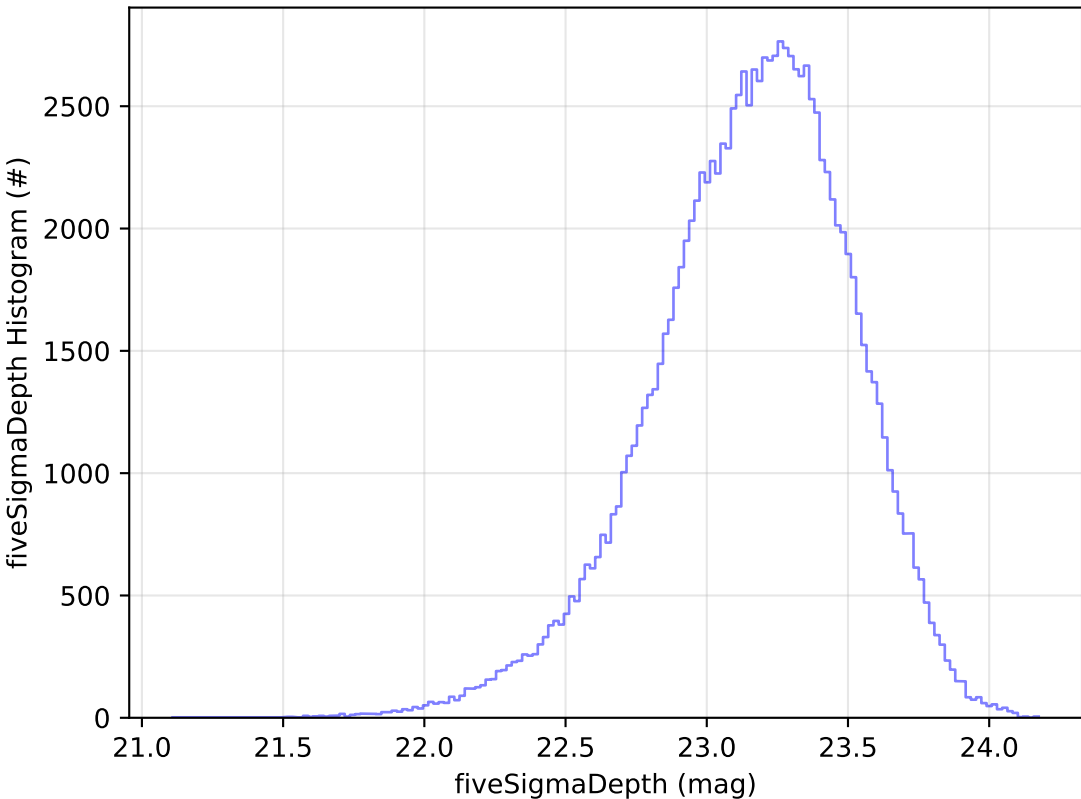
roll_uniform_early_half_mjdp253_v3.4_10yrs u: fiveSigmaDepth Histogram
