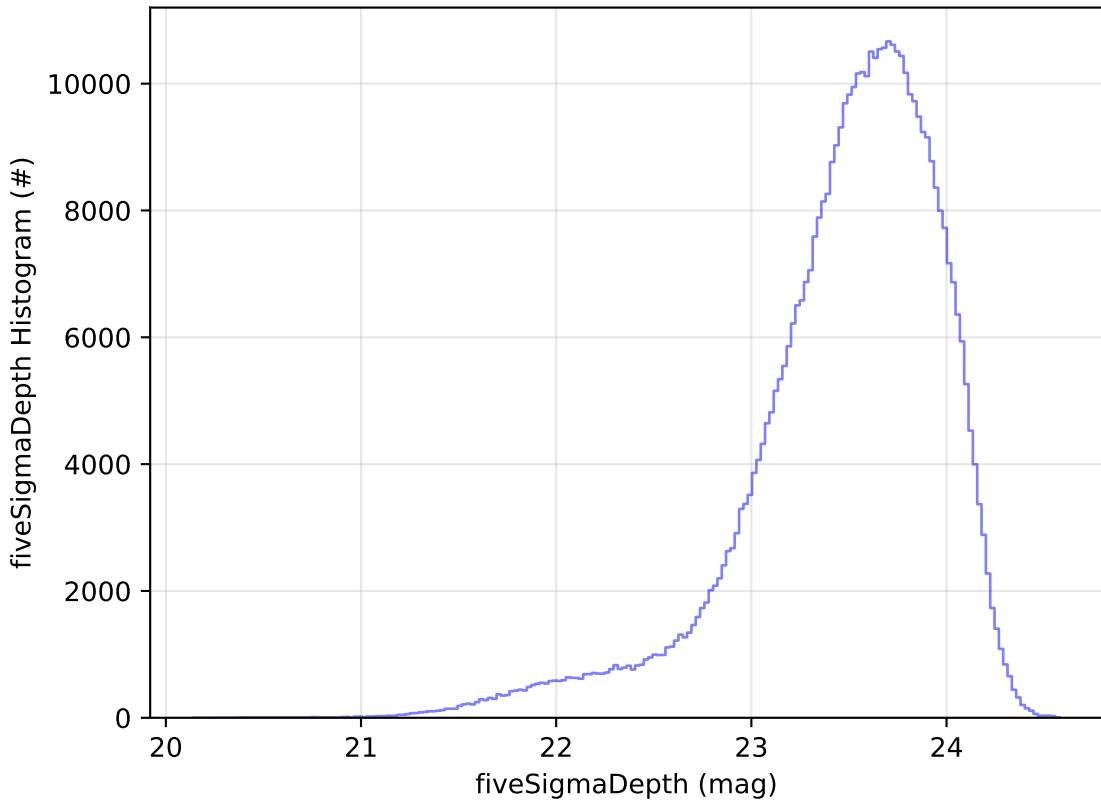
roll_uniform_early_half_mjdp253_v3.4_10yrs i: fiveSigmaDepth Histogram
