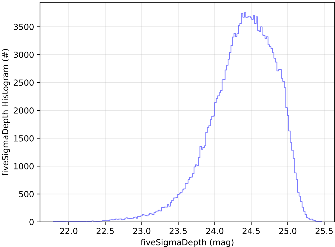
roll_uniform_early_half_mjdp253_v3.4_10yrs g: fiveSigmaDepth Histogram
