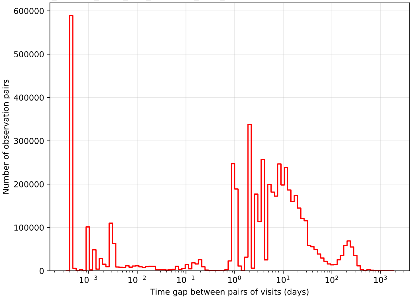
roll_uniform_early_half_mjdp253_v3.4_10yrs i band: Tgaps observationStartMJD
