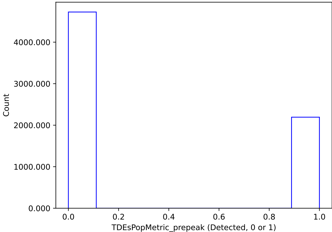
roll_uniform_early_half_mjdp253_v3.4_10yrs : TDEsPopMetric_prepeak
