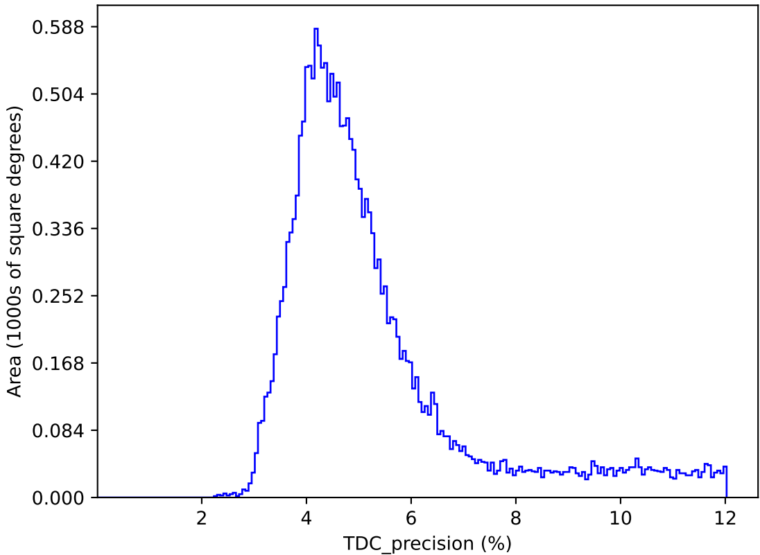
roll_uniform_early_half_mjdp253_v3.4_10yrs : TDC_precision
