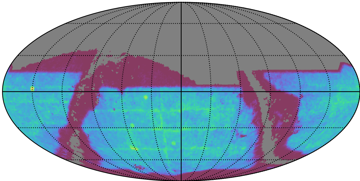
roll_uniform_early_half_mjdp253_v3.4_10yrs : SNSLMetric
