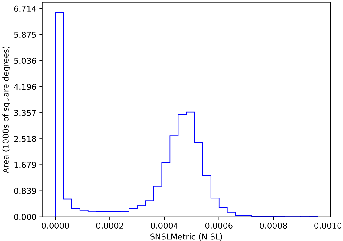
roll_uniform_early_half_mjdp253_v3.4_10yrs : SNSLMetric
