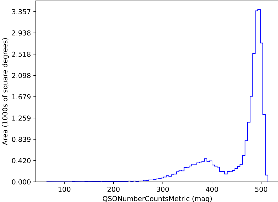
roll_uniform_early_half_mjdp253_v3.4_10yrs z band and non-DD: QSONumberCountsMetric
