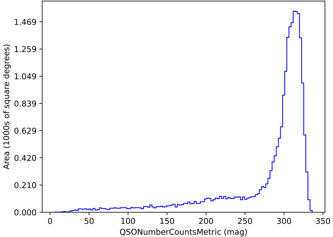
roll_uniform_early_half_mjdp253_v3.4_10yrs u band and non-DD: QSONumberCountsMetric
