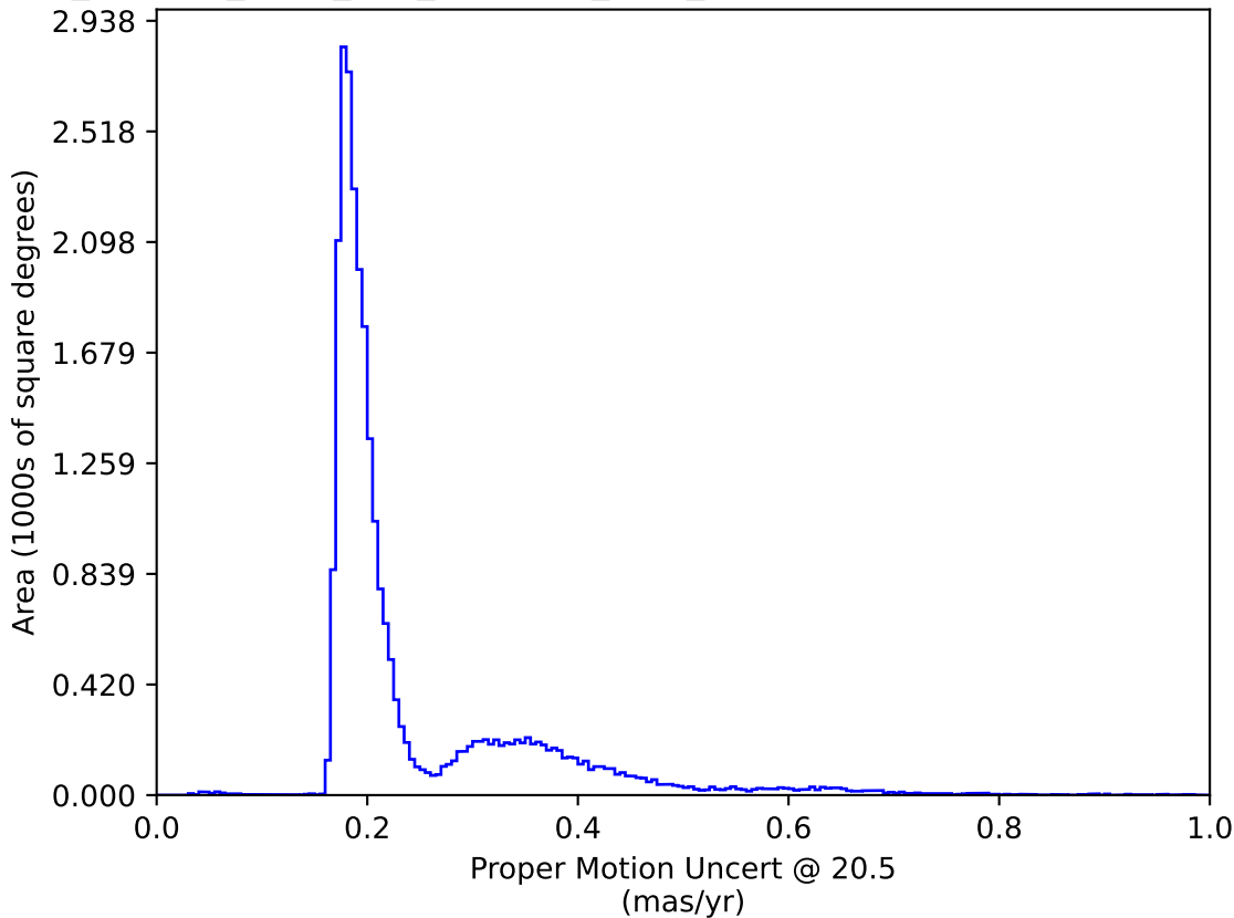
roll_uniform_early_half_mjdp253_v3.4_10yrs : Proper Motion Uncert @ 20.5
