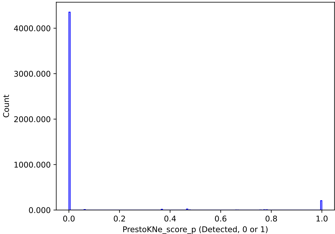
roll_uniform_early_half_mjdp253_v3.4_10yrs : PrestoKNe_score_p
