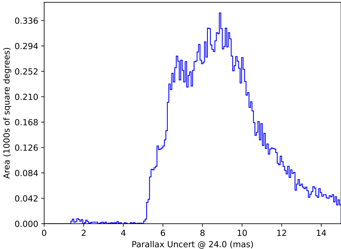
roll_uniform_early_half_mjdp253_v3.4_10yrs : Parallax Uncert @ 24.0
