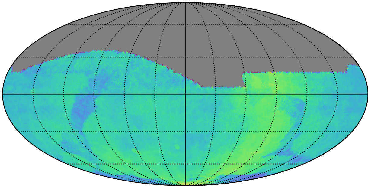
roll_uniform_early_half_mjdp253_v3.4_10yrs : Parallax Coverage @ 22.4
