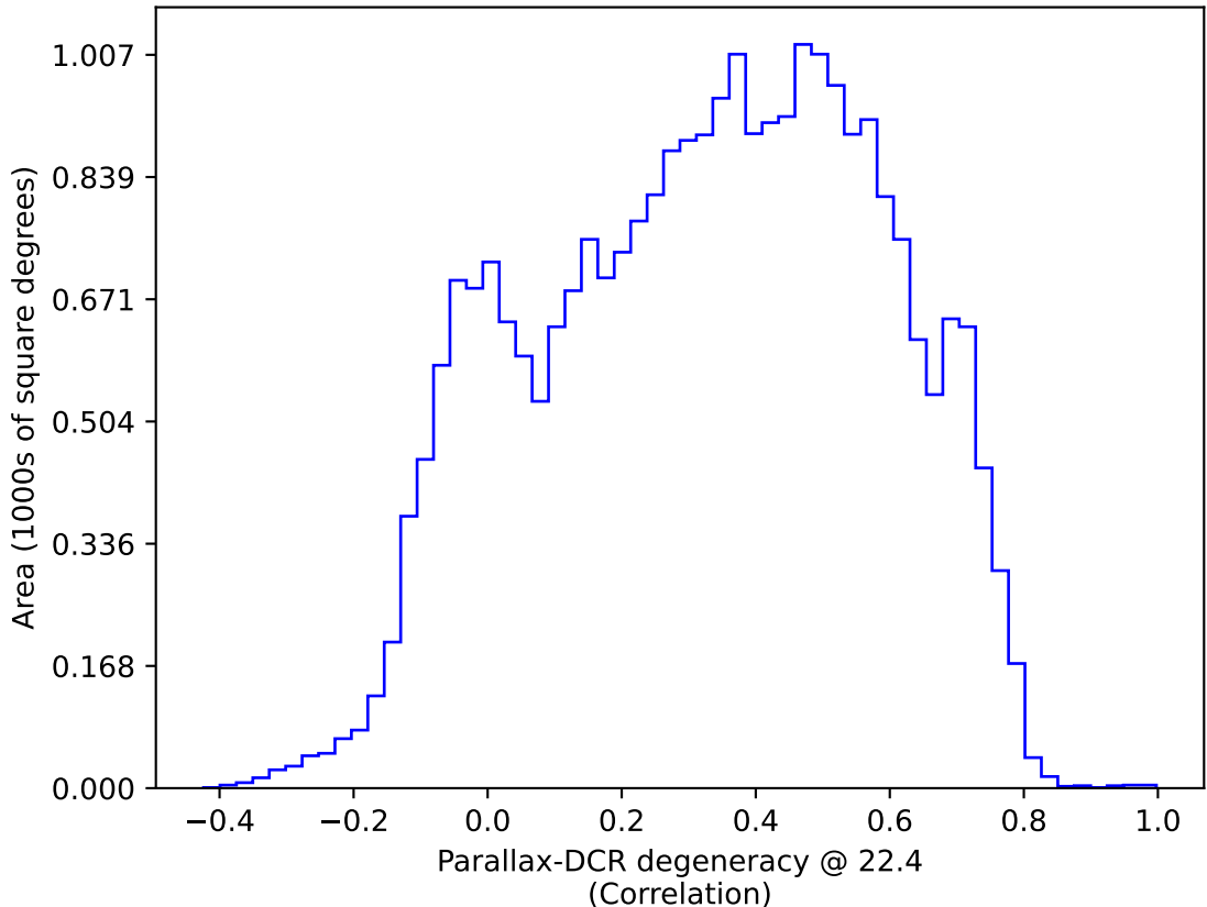
roll_uniform_early_half_mjdp253_v3.4_10yrs : Parallax-DCR degeneracy @ 22.4
