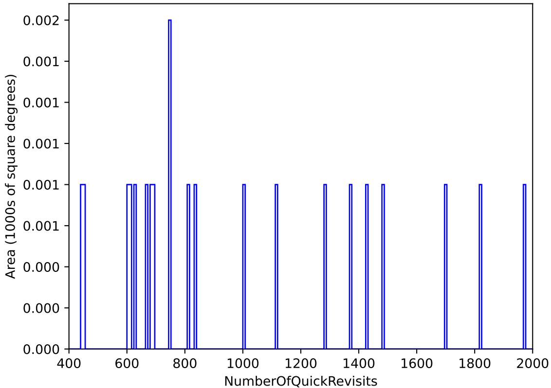
roll_uniform_early_half_mjdp253_v3.4_10yrs : NumberOfQuickRevisits
