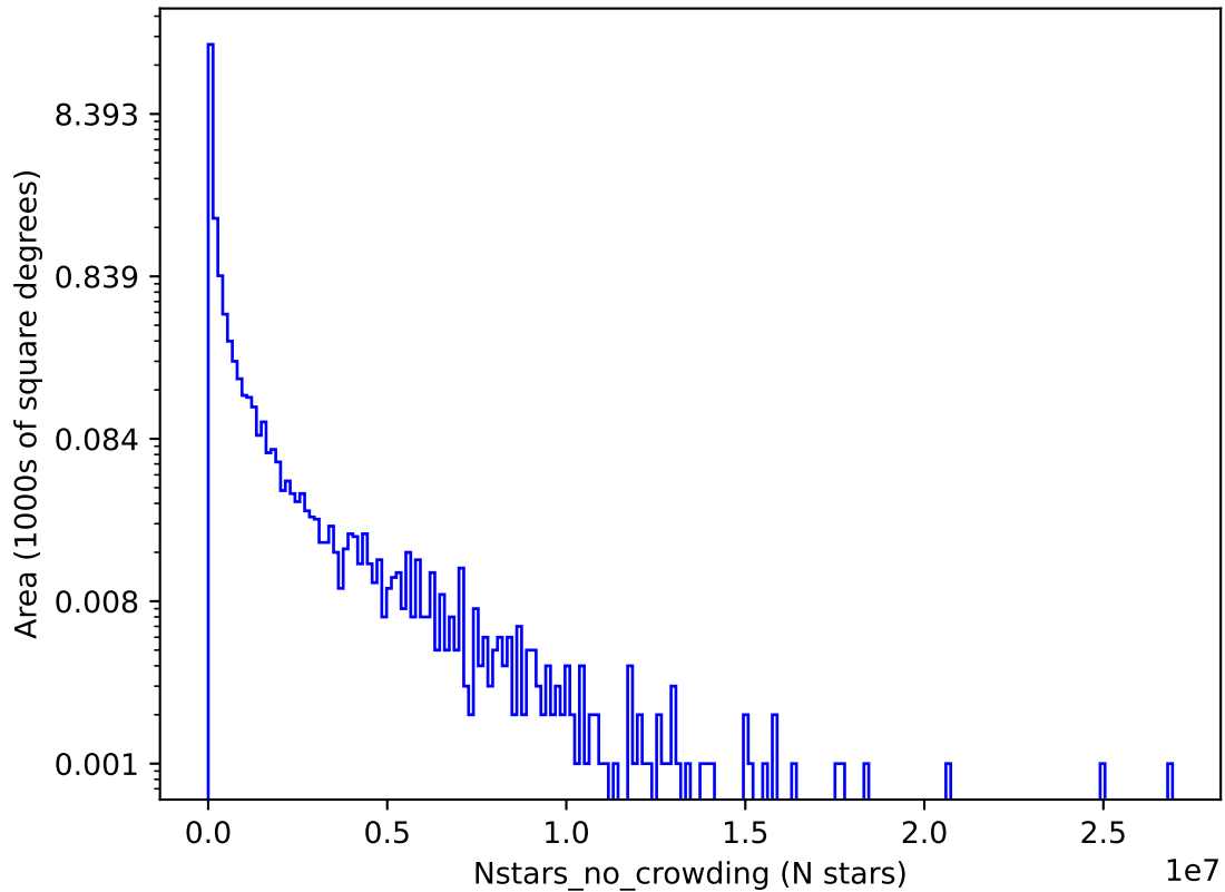
roll_uniform_early_half_mjdp253_v3.4_10yrs i: Nstars_no_crowding
