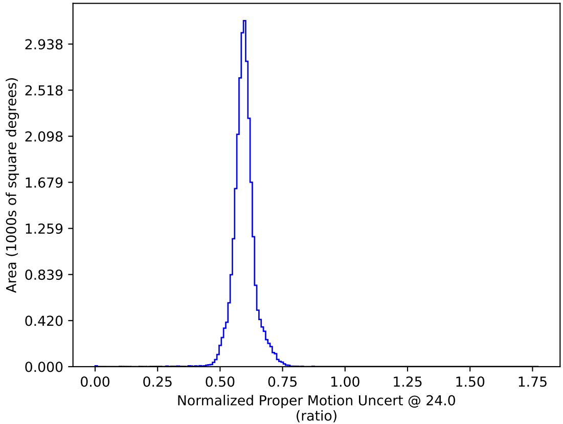
roll_uniform_early_half_mjdp253_v3.4_10yrs : Normalized Proper Motion Uncert @ 24.0
