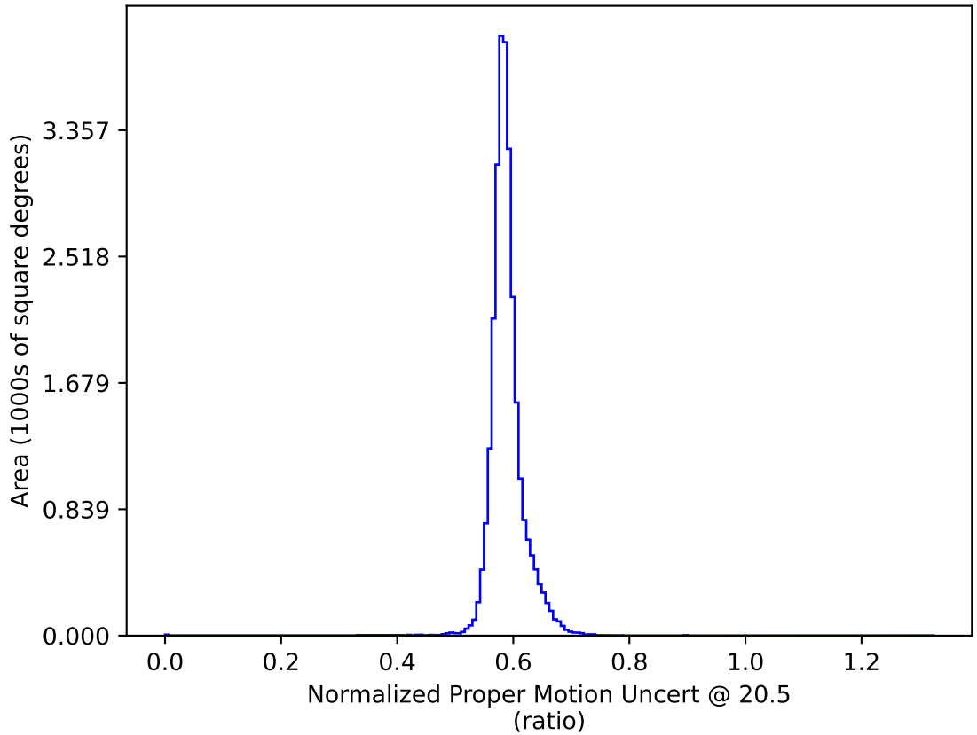
roll_uniform_early_half_mjdp253_v3.4_10yrs : Normalized Proper Motion Uncert @ 20.5
