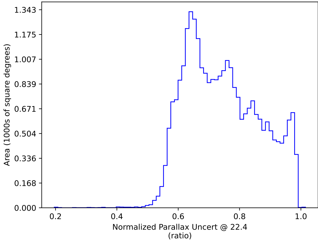
roll_uniform_early_half_mjdp253_v3.4_10yrs : Normalized Parallax Uncert @ 22.4
