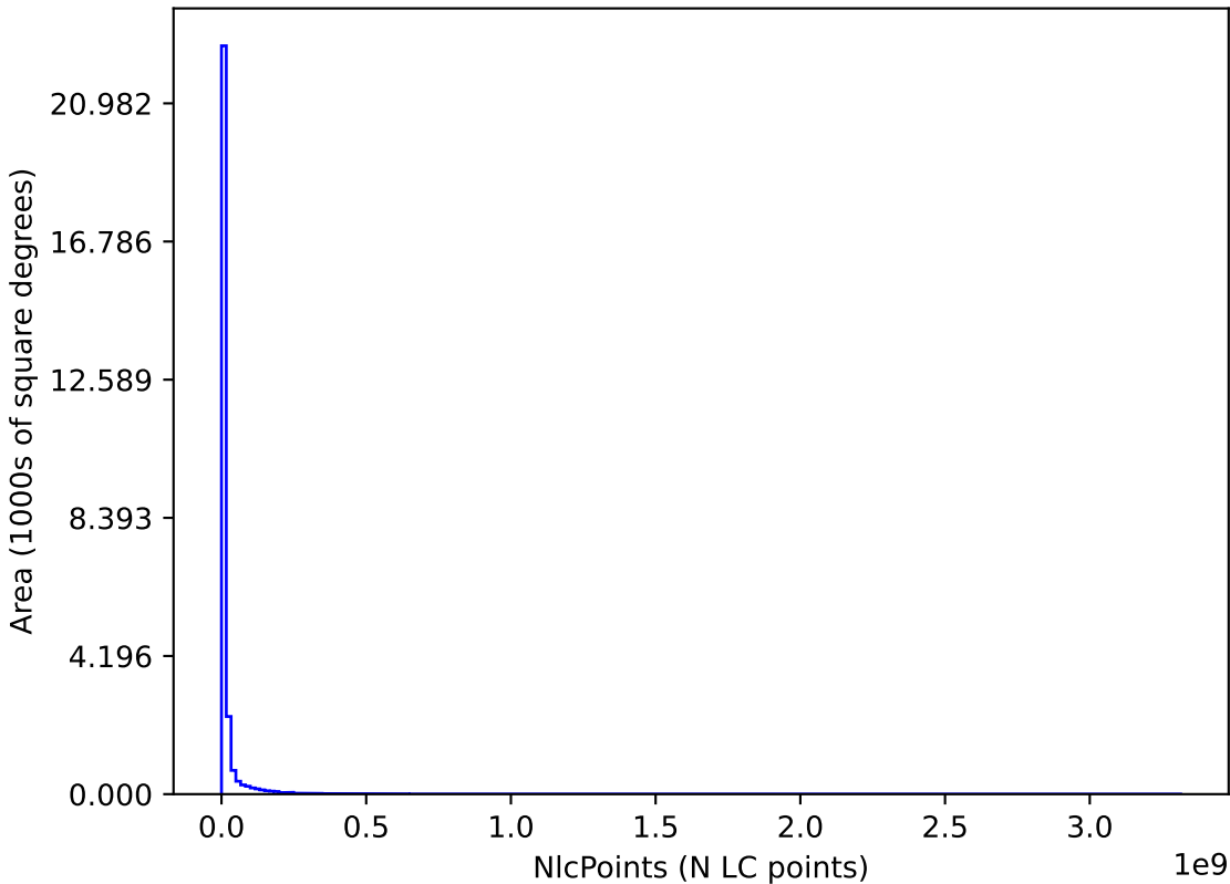
roll_uniform_early_half_mjdp253_v3.4_10yrs : NlcPoints
