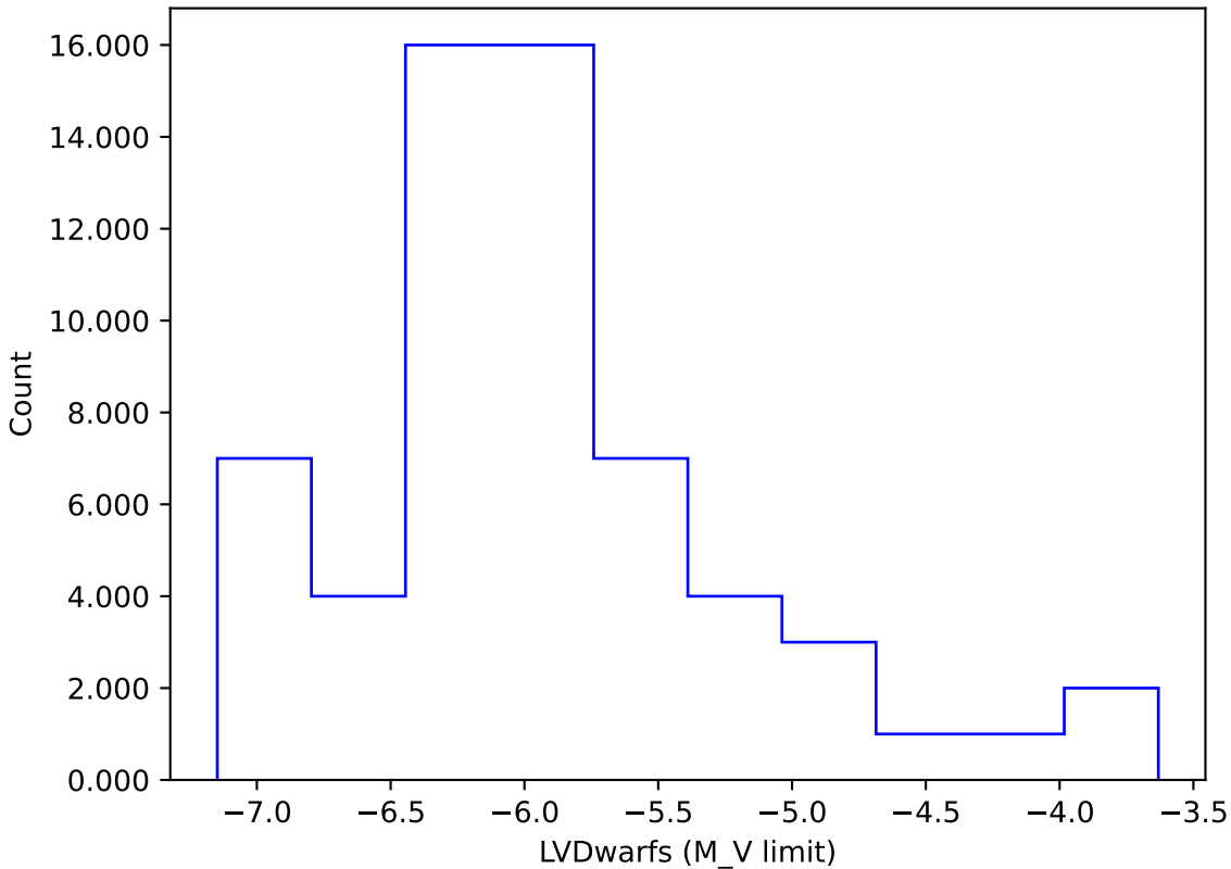
roll_uniform_early_half_mjdp253_v3.4_10yrs gi: LVDwarfs
