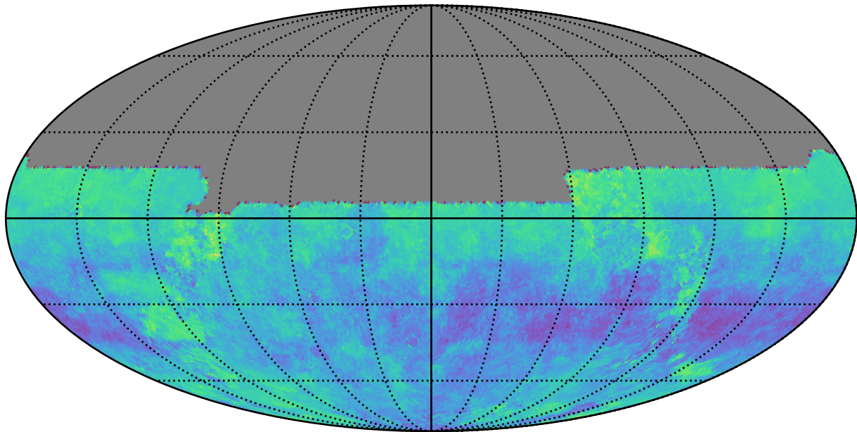
roll_uniform_early_half_mjdp253_v3.4_10yrs u: Kuiper rotSkyPos
