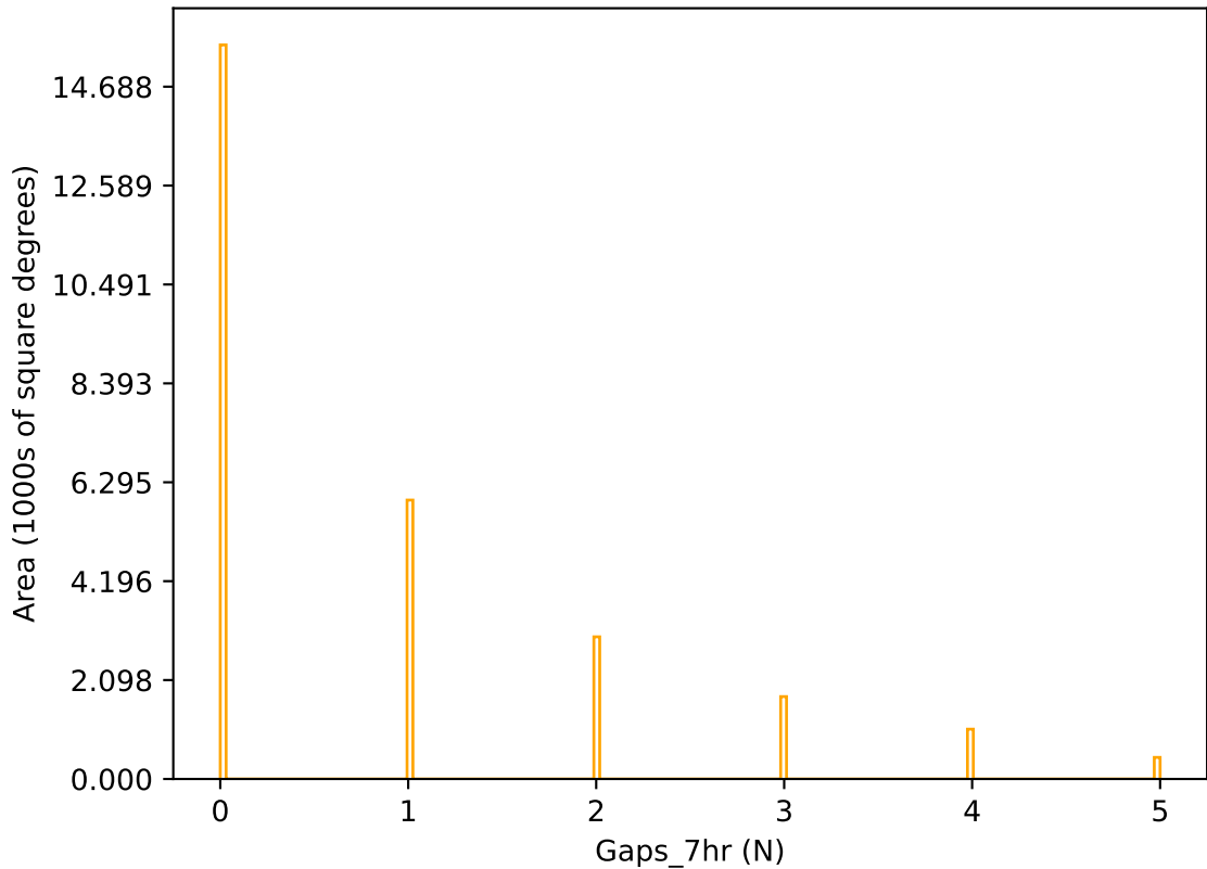
roll_uniform_early_half_mjdp253_v3.4_10yrs r band: Gaps_7hr
