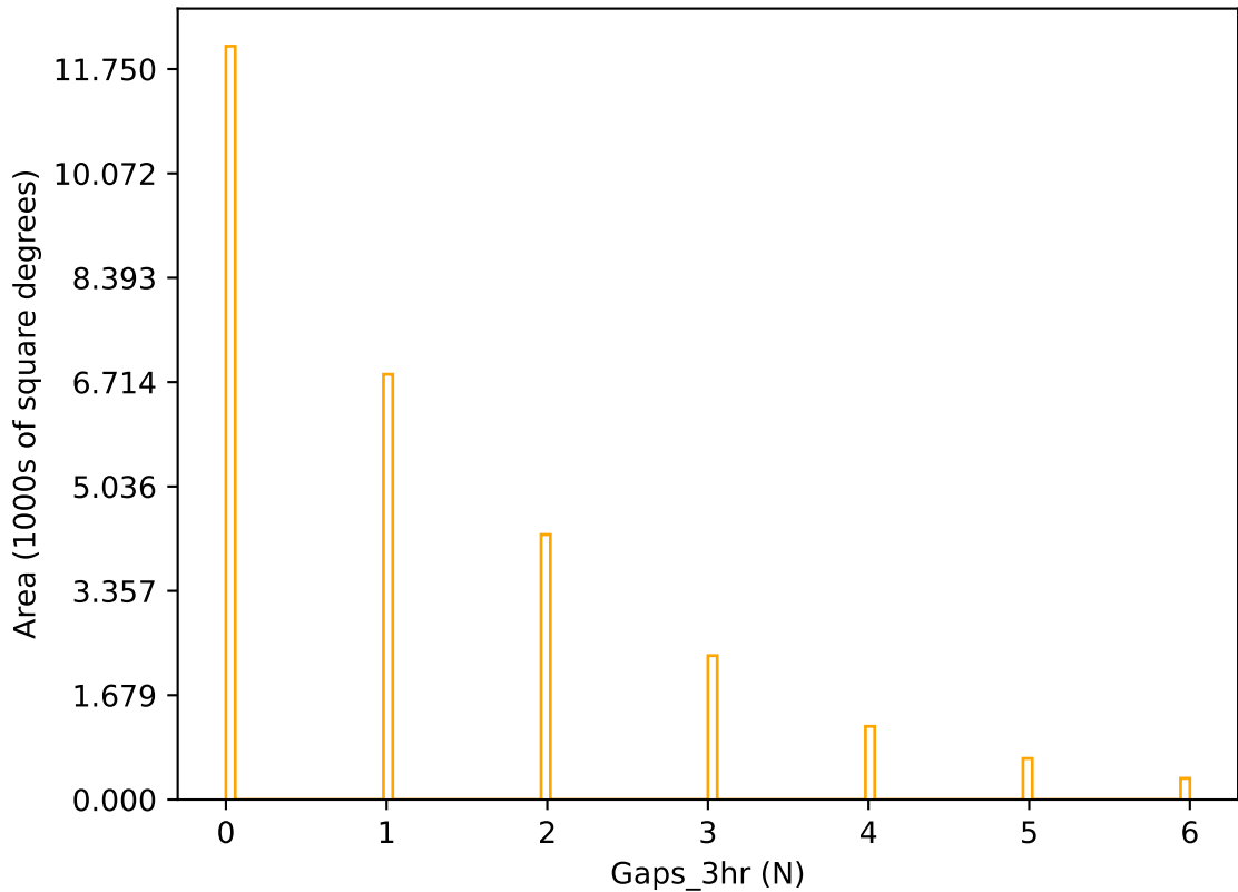
roll_uniform_early_half_mjdp253_v3.4_10yrs r band: Gaps_3hr
