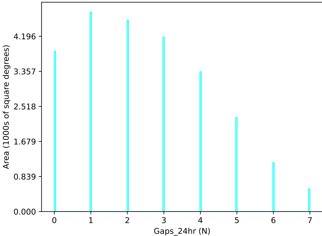
roll_uniform_early_half_mjdp253_v3.4_10yrs u band: Gaps_24hr
