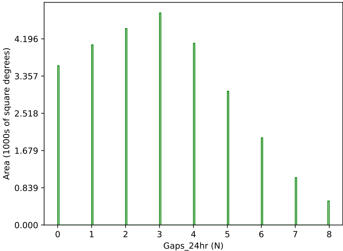
roll_uniform_early_half_mjdp253_v3.4_10yrs g band: Gaps_24hr
