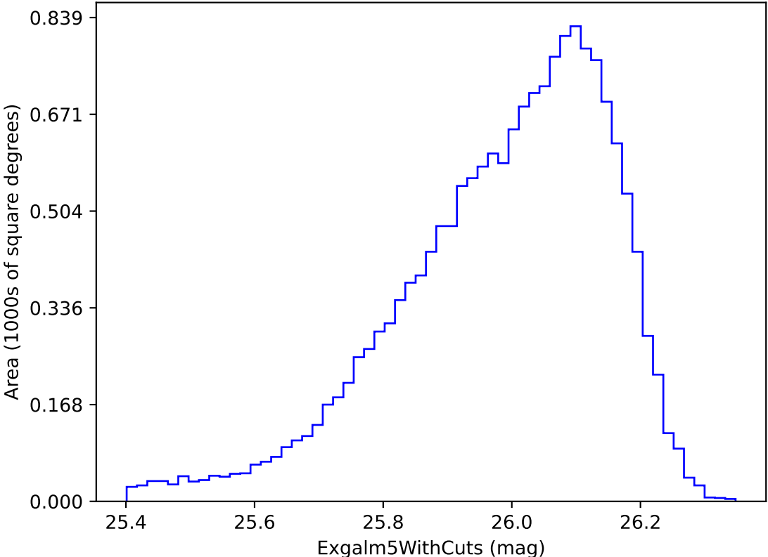
roll_uniform_early_half_mjdp253_v3.4_10yrs i band non-DD year 4: ExgalM5WithCuts
