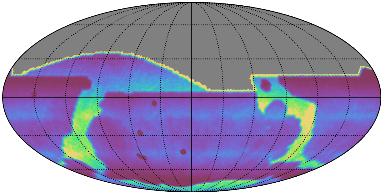
roll_uniform_early_half_mjdp253_v3.4_10yrs : DCRprecision
