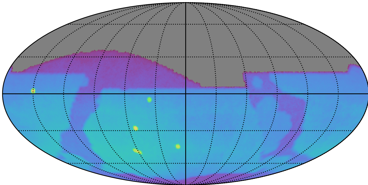
roll_uniform_early_half_mjdp253_v3.4_10yrs : Brown Dwarf, L7
