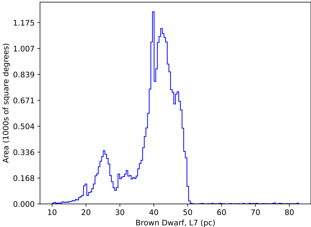
roll_uniform_early_half_mjdp253_v3.4_10yrs : Brown Dwarf, L7
