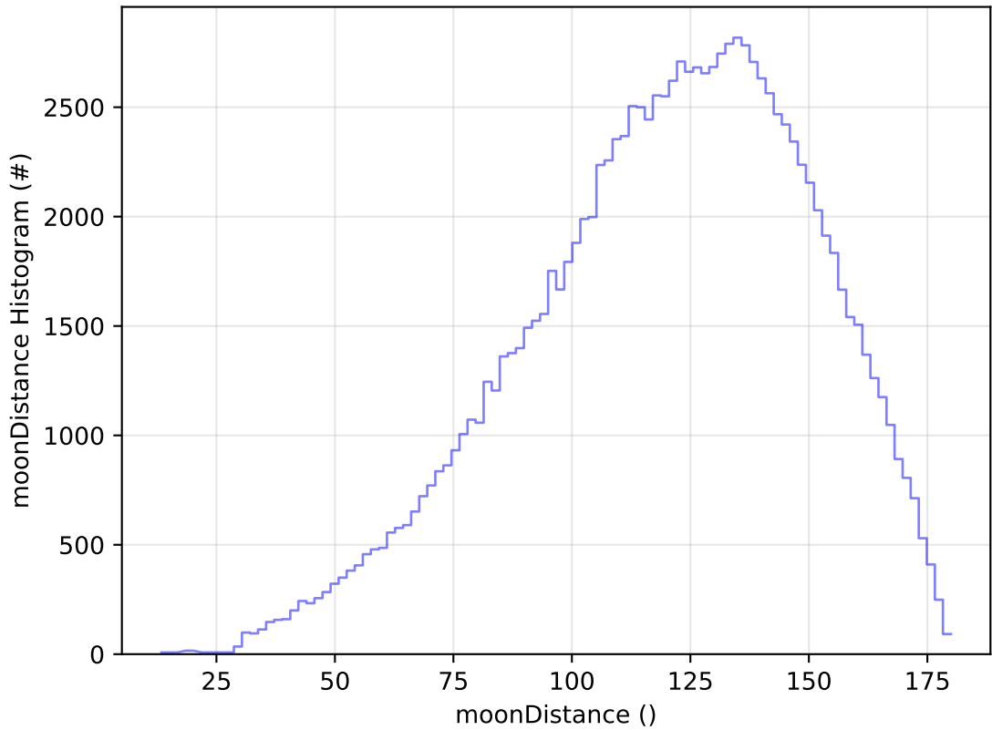
roll_uniform_early_half_mjdp253_v3.4_10yrs WFD u band: moonDistance Histogram
