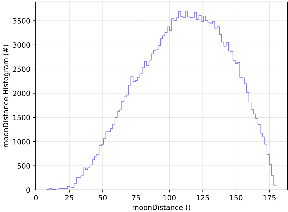
roll_uniform_early_half_mjdp253_v3.4_10yrs WFD g band: moonDistance Histogram
