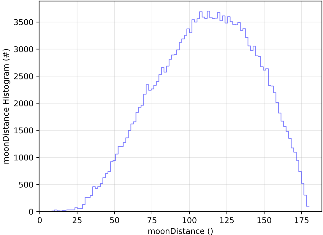
roll_uniform_early_half_mjdp253_v3.4_10yrs All sky g band: moonDistance Histogram
