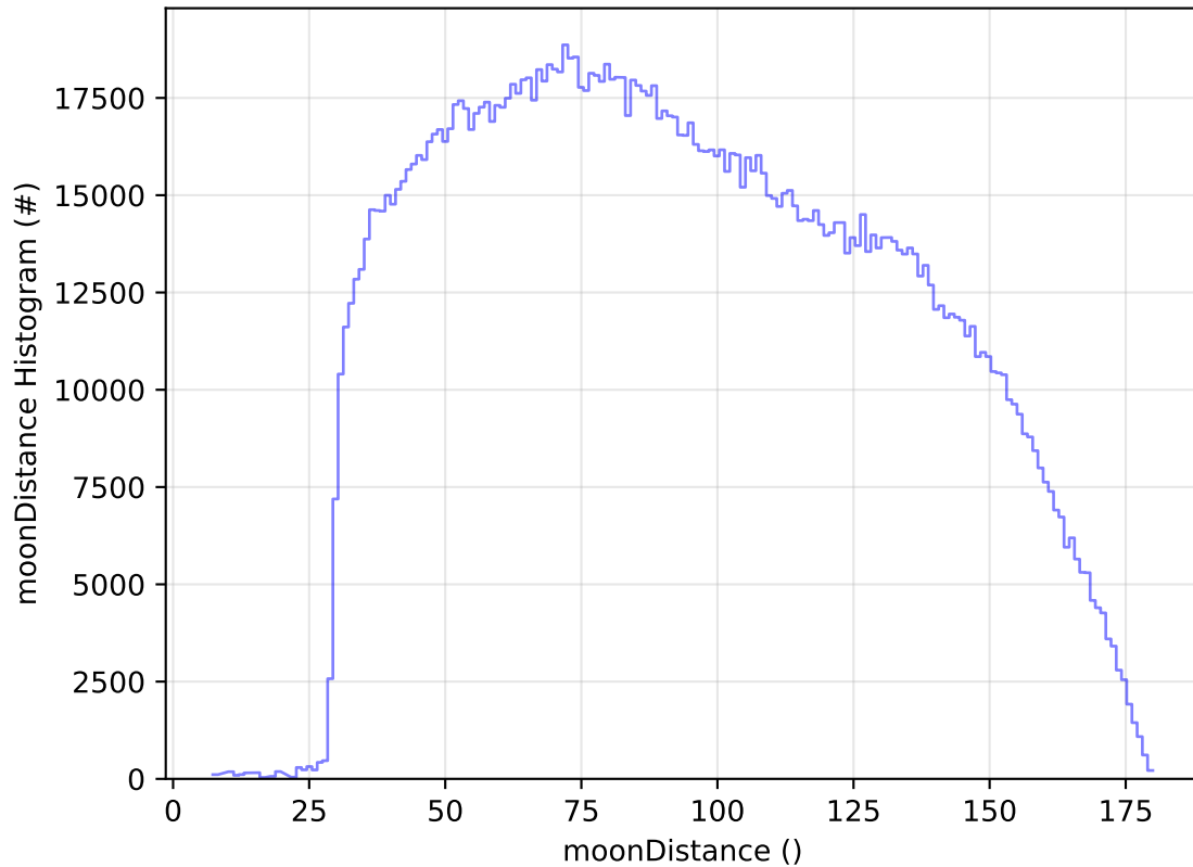
roll_uniform_early_half_mjdp253_v3.4_10yrs All sky all bands: moonDistance Histogram
