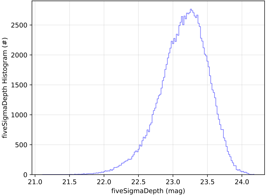
roll_uniform_early_half_mjdp253_v3.4_10yrs All sky u band: fiveSigmaDepth Histogram
