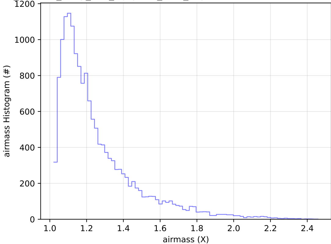
roll_uniform_early_half_mjdp253_v3.4_10yrs Yr 1 u band: airmass Histogram
