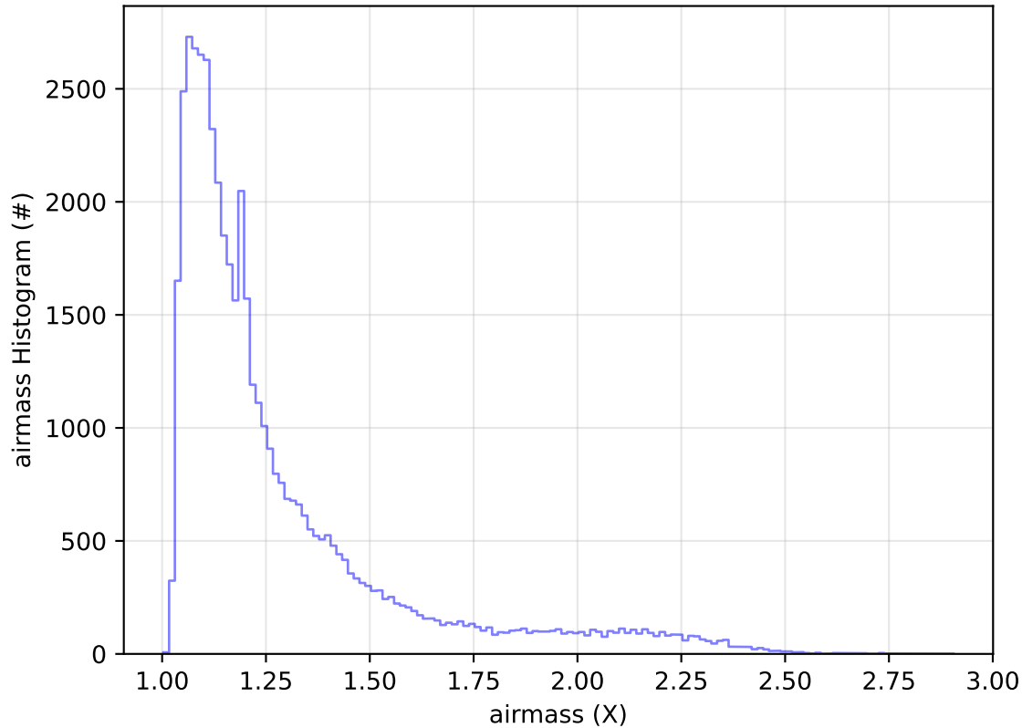
roll_uniform_early_half_mjdp253_v3.4_10yrs Yr 1 r band: airmass Histogram
