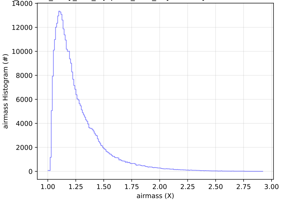
roll_uniform_early_half_mjdp253_v3.4_10yrs WFD y band: airmass Histogram
