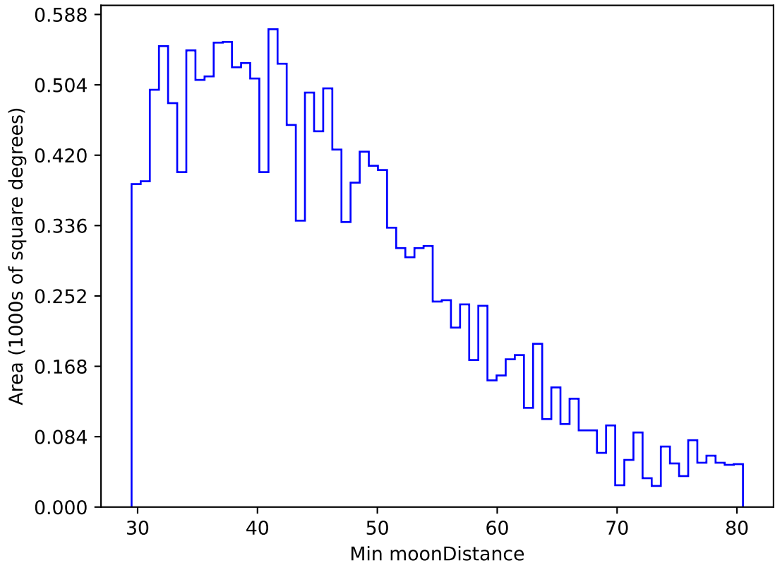
roll_uniform_early_half_mjdp253_v3.4_10yrs WFD g band: Min moonDistance
