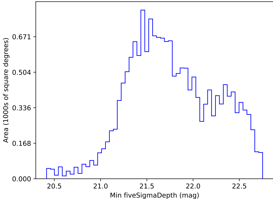
roll_uniform_early_half_mjdp253_v3.4_10yrs WFD i band: Min fiveSigmaDepth
