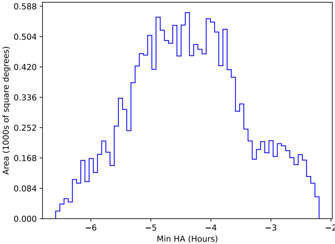
roll_uniform_early_half_mjdp253_v3.4_10yrs WFD z band: Min HA
