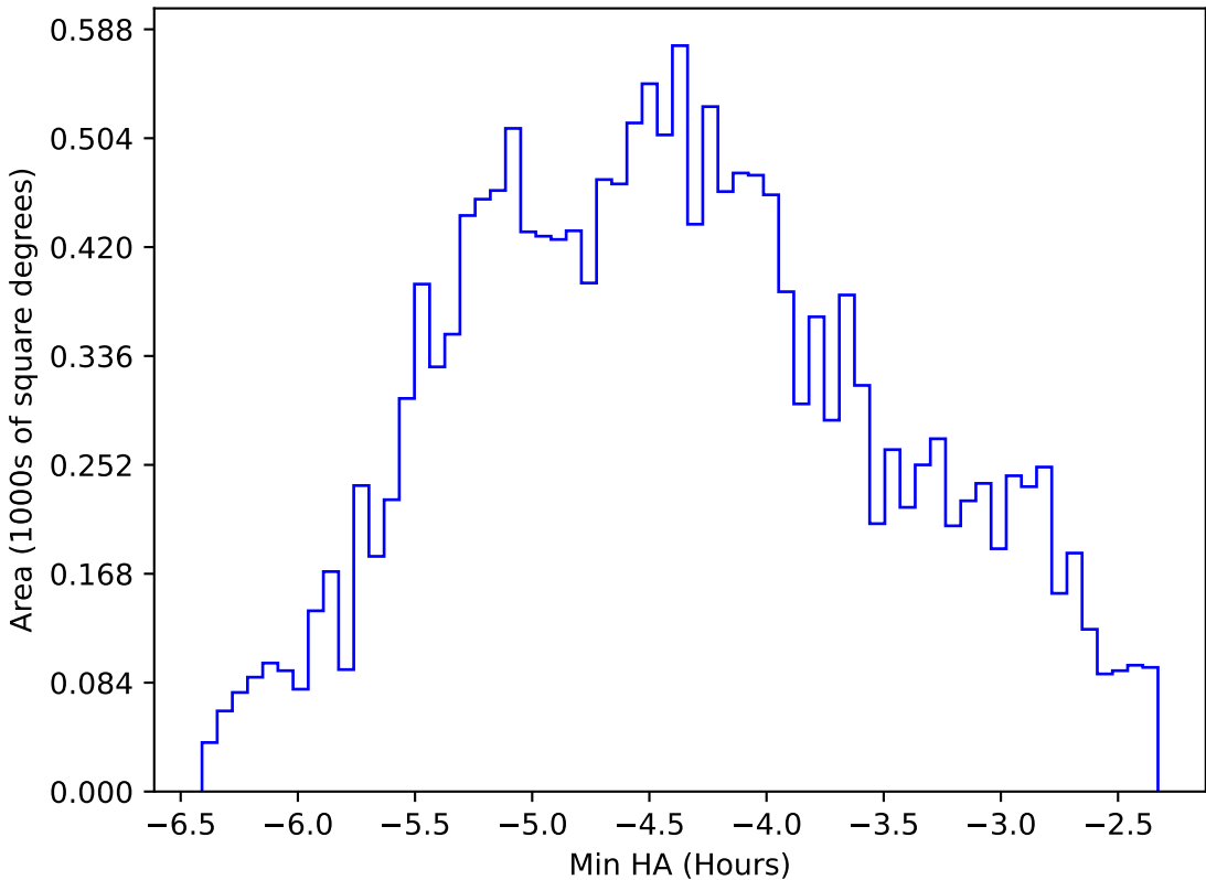
roll_uniform_early_half_mjdp253_v3.4_10yrs WFD r band: Min HA
