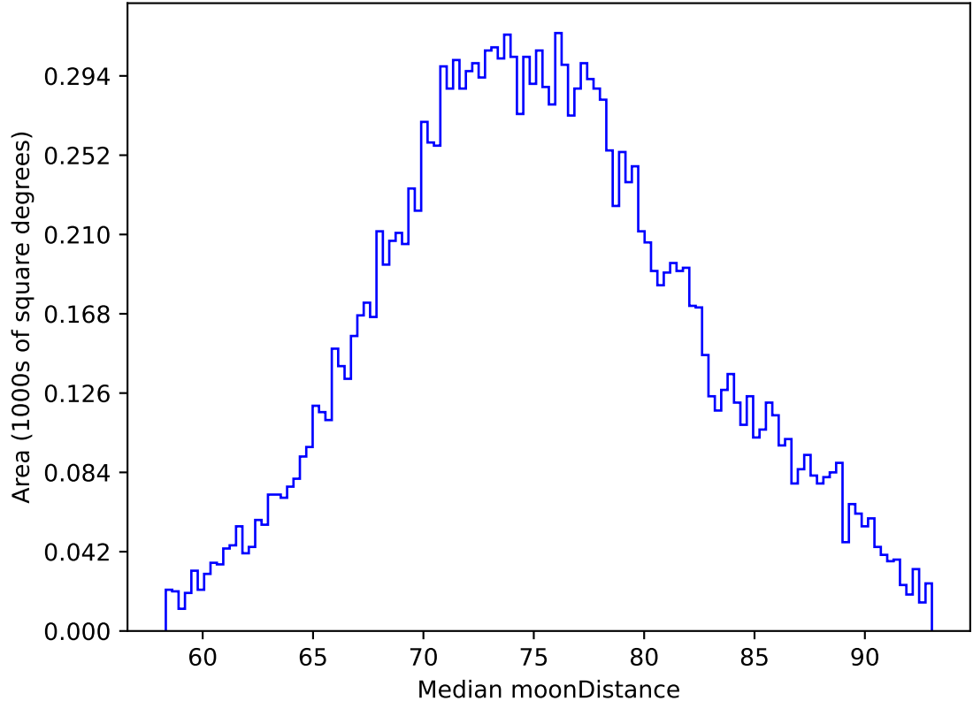
roll_uniform_early_half_mjdp253_v3.4_10yrs WFD z band: Median moonDistance
