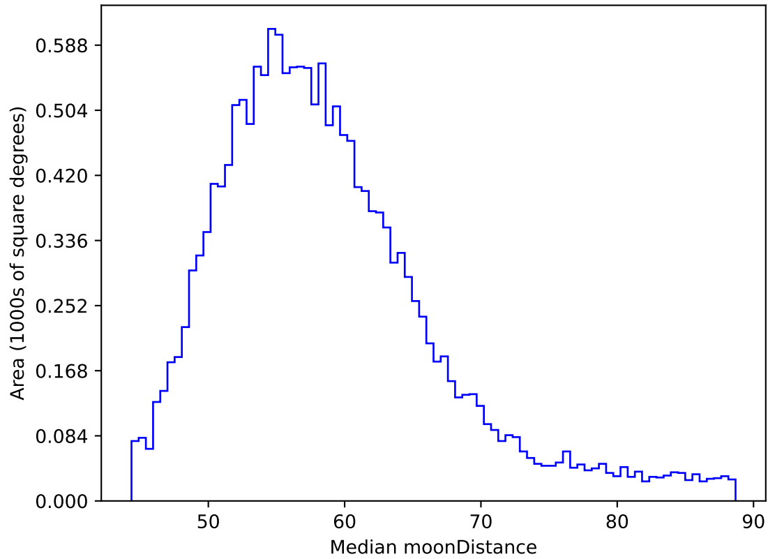
roll_uniform_early_half_mjdp253_v3.4_10yrs WFD y band: Median moonDistance
