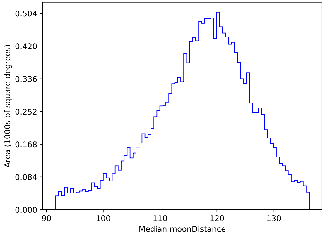
roll_uniform_early_half_mjdp253_v3.4_10yrs WFD g band: Median moonDistance
